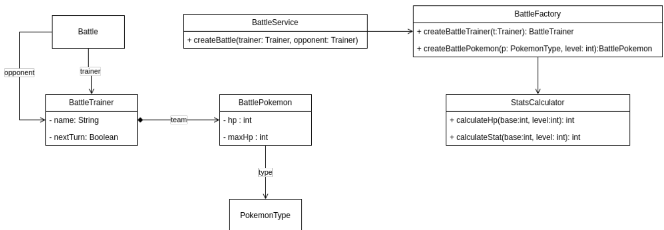
Figure 1. Battle UML
